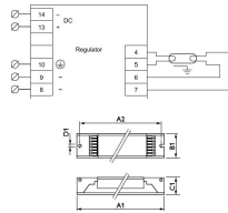
Specificaties Philips HF-R 136 TL-D EII 220-240V
